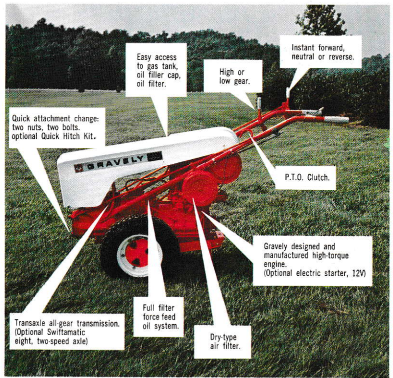
7.6 HP TRACTOR
