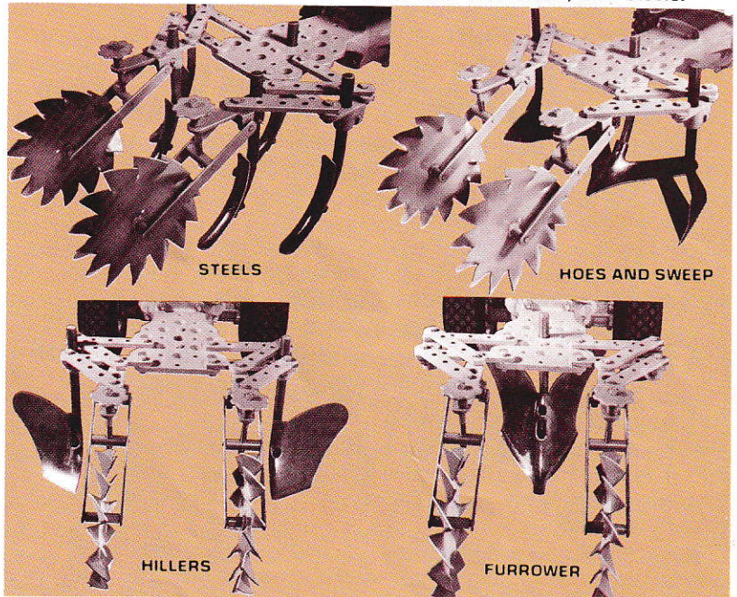
TOOL SET-UPS FOR TOOLHOLDERS
