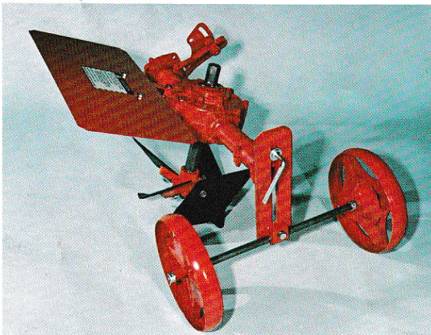
Gravelly 7.6 HP Super Convertible Tractor with Rotary Plow
